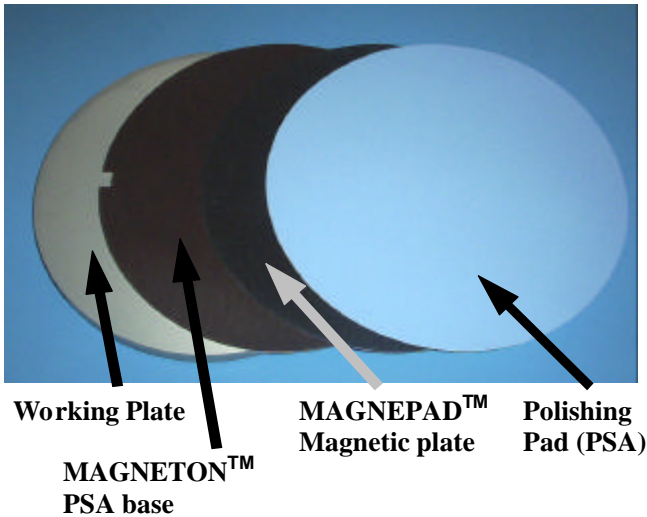
Figure 1a. Magnetic Polishing System using standard PSA backed polishing pads.
